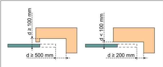
Illustration 1: Safety distance
