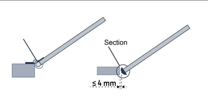
Illustration 2: Mechanical protection
