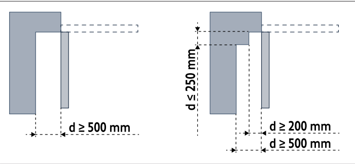
Illustration 1: Safety distances
