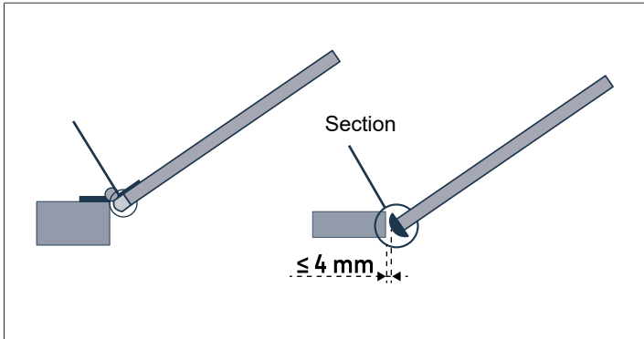
Illustration 2: Mechanical protection
