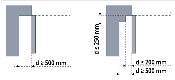
Illustration 1: Safety distances
